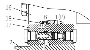
Illustration: directional valve opened
