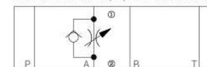
Model Z2FS6A-...-4XJ/...(meter-out control)
