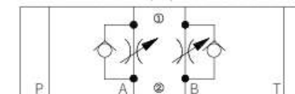
Model Z2FS6-...-4XJ/...(meter-out control)
