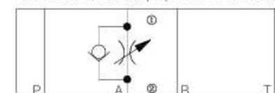
Model Z2FS6A-...-4XJ/...(meter-in control)
