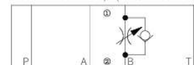
Model Z2FS6B-...-4XJ/...(meter-in control)
