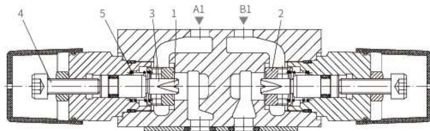
Model Z2FS6-2-4XJ/(meter-in control)
