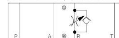
Model Z2FS6B-...-4XJ/...(meter-out control)
