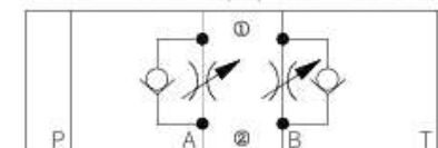
Model Z2FS6-...-4XJ/...(meter-in control)
